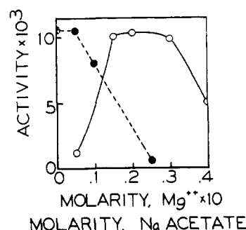
FIG. 5.—Effect of buffer and \text{Mg}^{++} concentrations on the activity of venom endonuclease. Kunitz's spectrophotometric method was used. For the determination of the optimal buffer concentration, the reaction cells contained 3 ml DNA ( 0.04 \text{ mg/ml} in \text{H}_2\text{O} ), 0.05 \text{ ml} enzyme ( 0.01 \text{ unit} ), a calculated quantity of 1 \text{ M} sodium acetate buffer, pH 5.0, to attain the indicated molarity, and water to a total volume of 4 \text{ ml} . For the determination of the effect of \text{Mg}^{++} the reaction cells contained 3 ml DNA ( 0.04 \text{ mg/ml} ), 0.05 \text{ ml} enzyme, a calculated volume of 0.25 \text{ M} \text{MgCl}_2 to attain the indicated molarity, and water to a total volume of 4 \text{ ml} . O—O Effect of buffer, ●—● effect of \text{Mg}^{++} .
