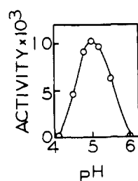
FIG. 4.—Effect of pH on activity of venom endonuclease. Kunitz's spectrophotometric method was used. The reaction cells contained 3 ml DNA solution ( 0.04 \text{ mg/ml} in \text{H}_2\text{O} ), 0.05 \text{ ml} enzyme solution ( 0.01 \text{ unit} ), 0.15 \text{ ml} \text{H}_2\text{O} , and 0.8 \text{ ml} 1 \text{ M} sodium acetate of the indicated pH.
