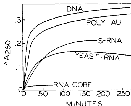
FIG. 6.—Digestion of various substrates with venom endonuclease. Kunitz's spectrophotometric method was used. The reaction mixtures contained 0.8 \text{ ml} 1 \text{ M} sodium acetate buffer, pH 5.0, 0.2 \text{ ml} enzyme solution (potency toward DNA 1.8), 3.0 \text{ ml} substrate. The concentrations of the various substrates in \text{A}_{260} units per ml of final reaction mixture were: DNA 1.96, Poly AU 1.75, yeast RNA 2.05, S-RNA 2.19, RNA core 2.7.
